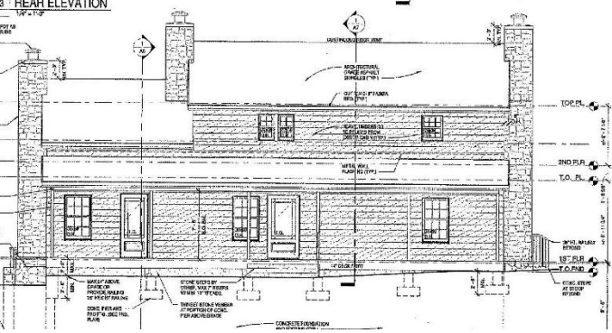
3 REAR ELEVATION
